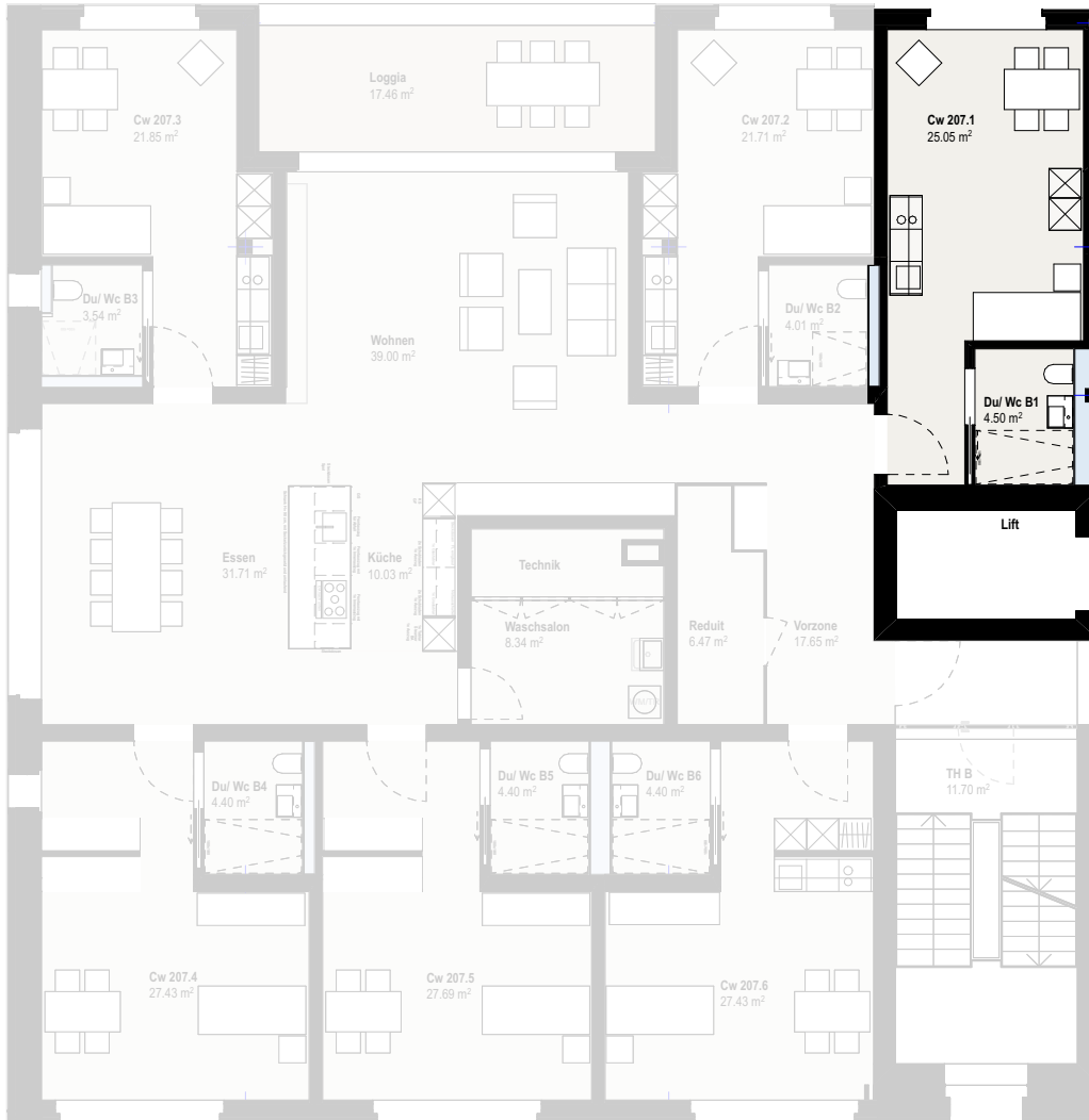
Cluster WG 207.1
